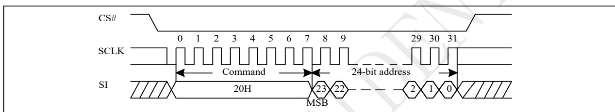
Figure 10-36 Sector Erase (SE) Sequence (SPI)
