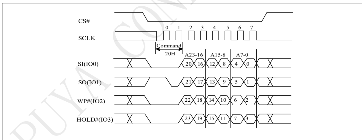
Figure 10-36a Sector Erase (SE) Sequence (QPI)
