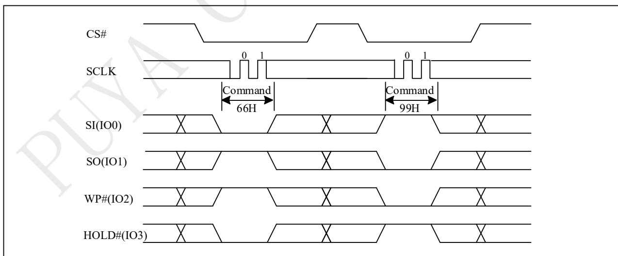
Figure 10-67b Software Reset Sequence (QPI)
