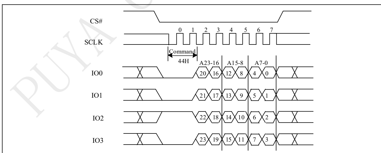
Figure 10-49a Erase Security Registers (ERSCUR) Sequence (QPI)
