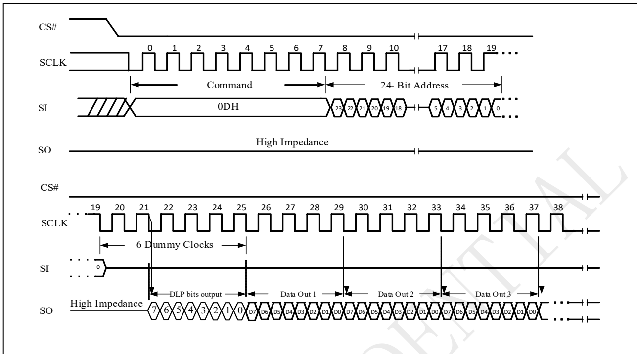
Figure 10-33g DTR 1IO Read with DLP bits output Sequence (SPI)
