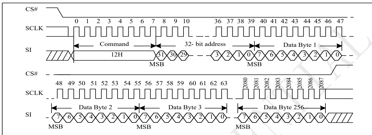
Figure 10-44 Page Program with 4-Byte Address Sequence (SPI)
