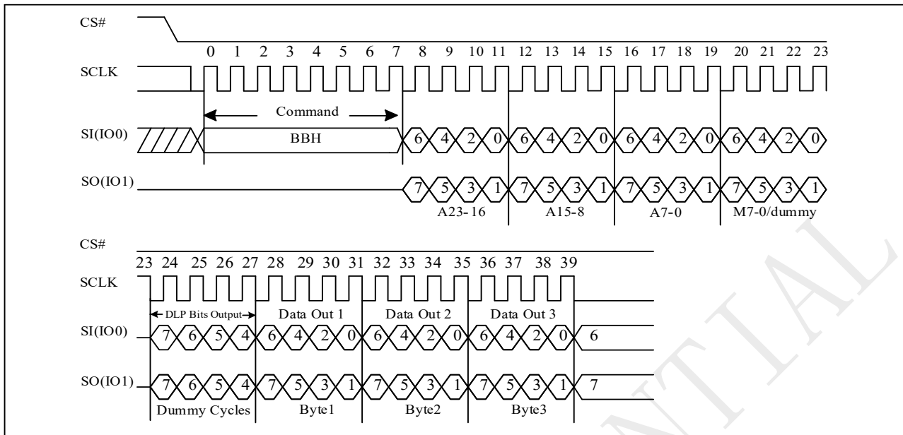
Figure 10-33d 2IO Read with DLP bits output Sequence (SPI)
