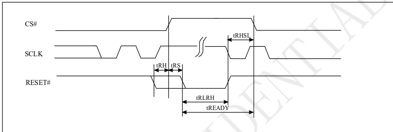
Figure 10-68 RESET Timing
