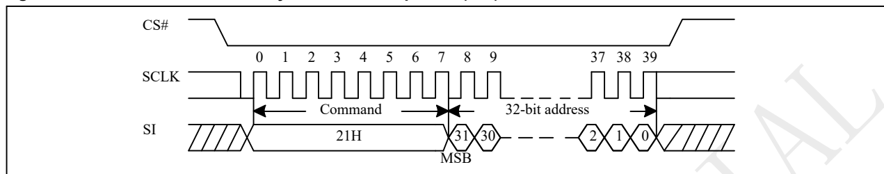
Figure 10-37 Sector Erase with 4-Byte Address Sequence (SPI)
