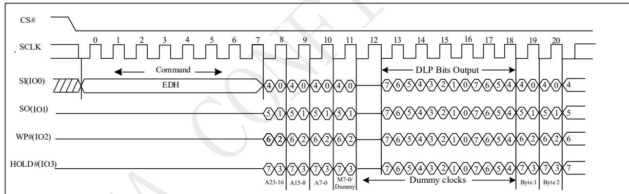
Figure 10-33j DTR 4IO Read with DLP bits output Sequence (SPI)
