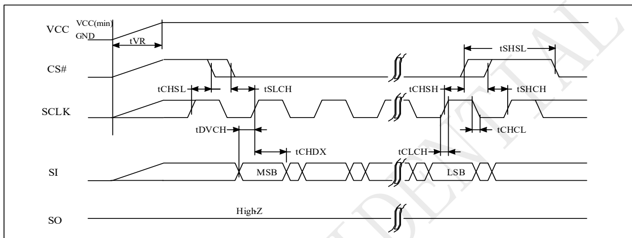
Figure 5-9 Power-up Timing
