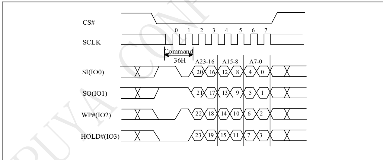
Figure 10-62a Individual Block Lock(QPI)
