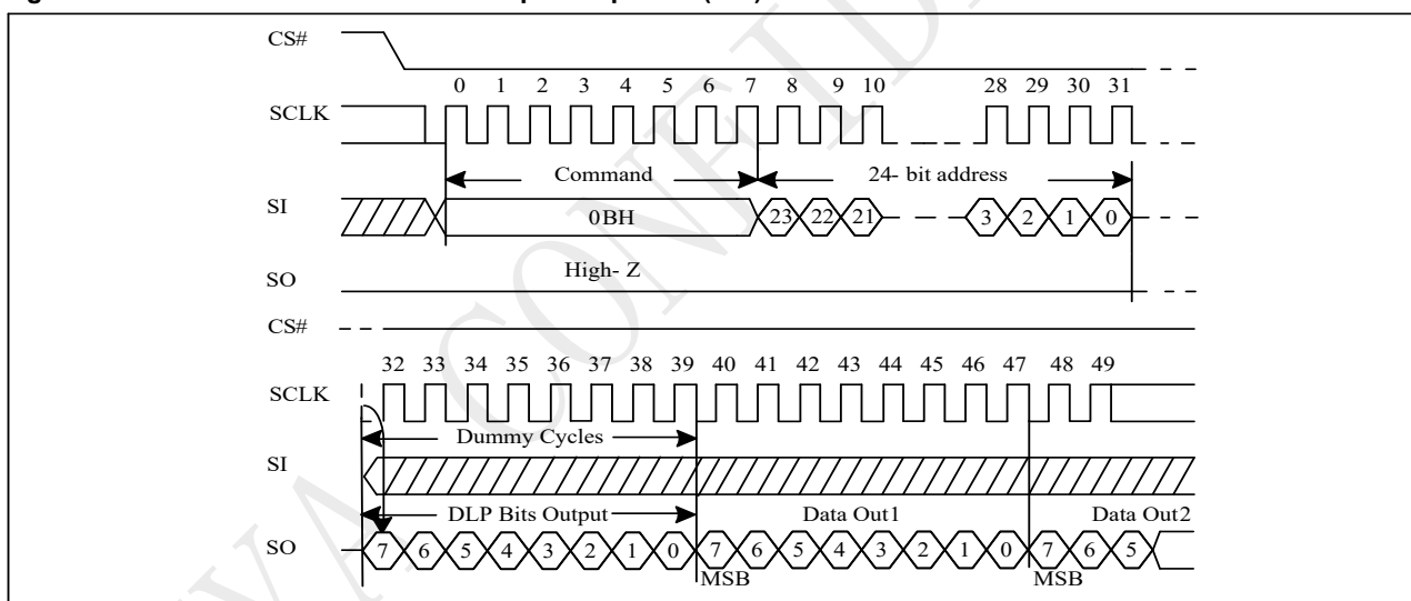
Figure 10-33 Fast Read with DLP bits output Sequence (SPI)
