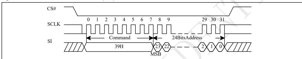
Figure 10-63 Individual Block Unlock (SPI)
