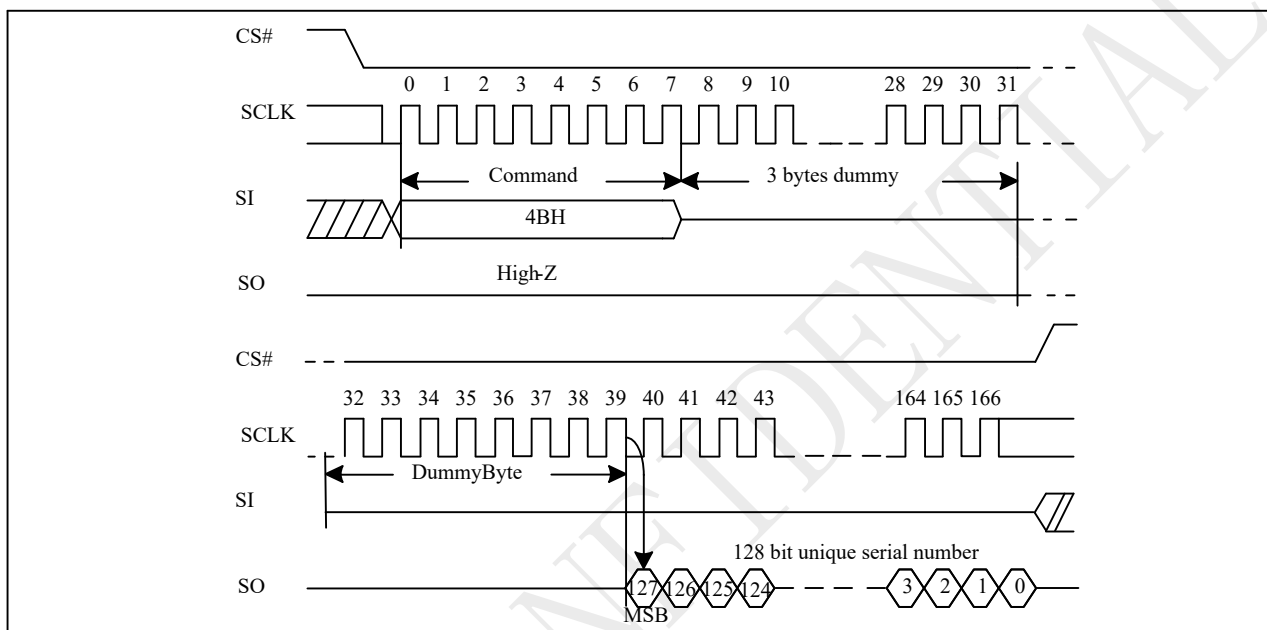
Figure 10-70 Read Unique ID (RUID) Sequence (SPI)
