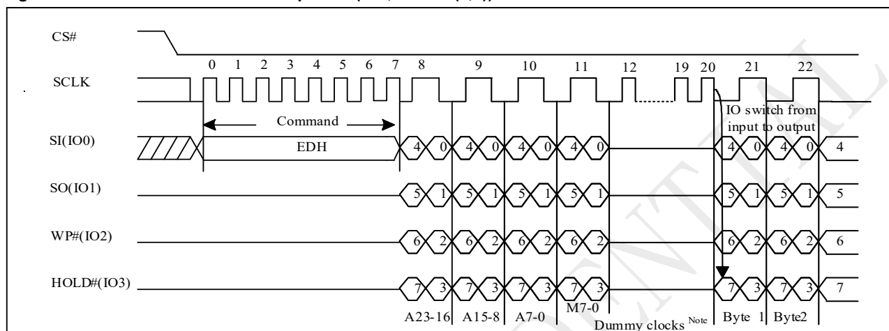
Figure 10-27 DTR 4IO Read Mode Sequence (SPI, M5-4 ≠ (1,0))
