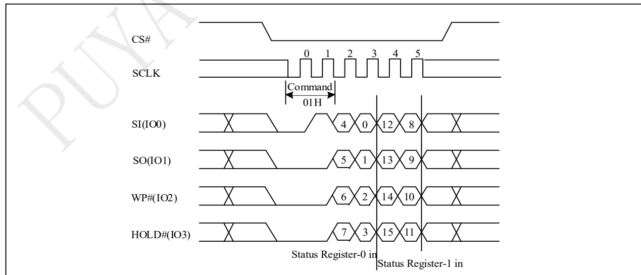
Figure 10-7c Write Status Register (WRSR) with 2 Byte data Sequence (QPI)
