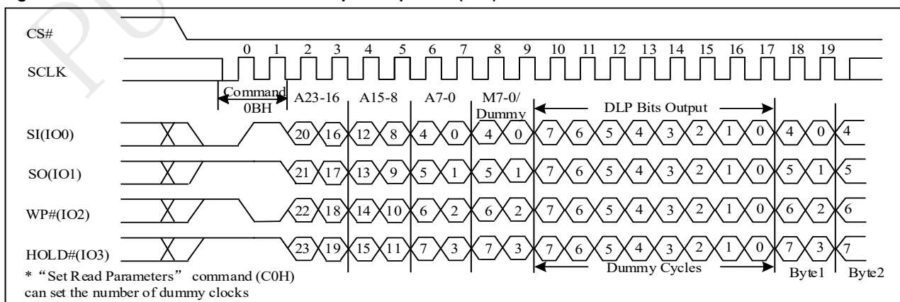
Figure 10-33a Fast Read with DLP bits output Sequence (QPI)
