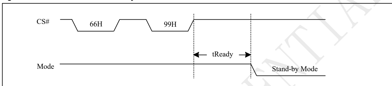
Figure 10-67a Software Reset Sequence (SPI)
