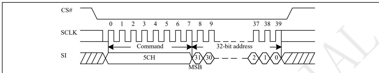
Figure 10-39 Block Erase 32K with 4-Byte Address (BE32K4B) Sequence (SPI)
