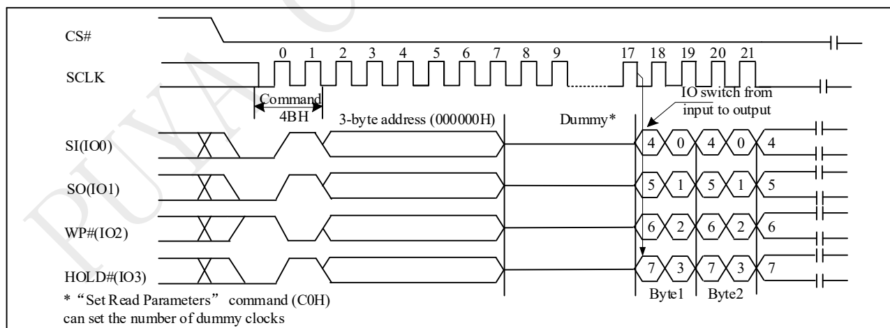
Figure 10-70a Read Unique ID (RUID) Sequence (QPI)
