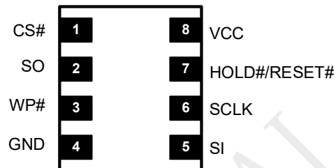
8-Pad WSON (6x5mm/8x6mm)
