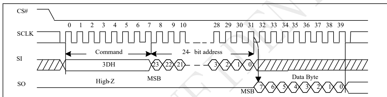
Figure 10-64 Read Block Lock Status (SPI)
