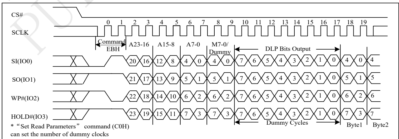
Figure 10-33f 4IO Read with DLP bits output Sequence (QPI)
