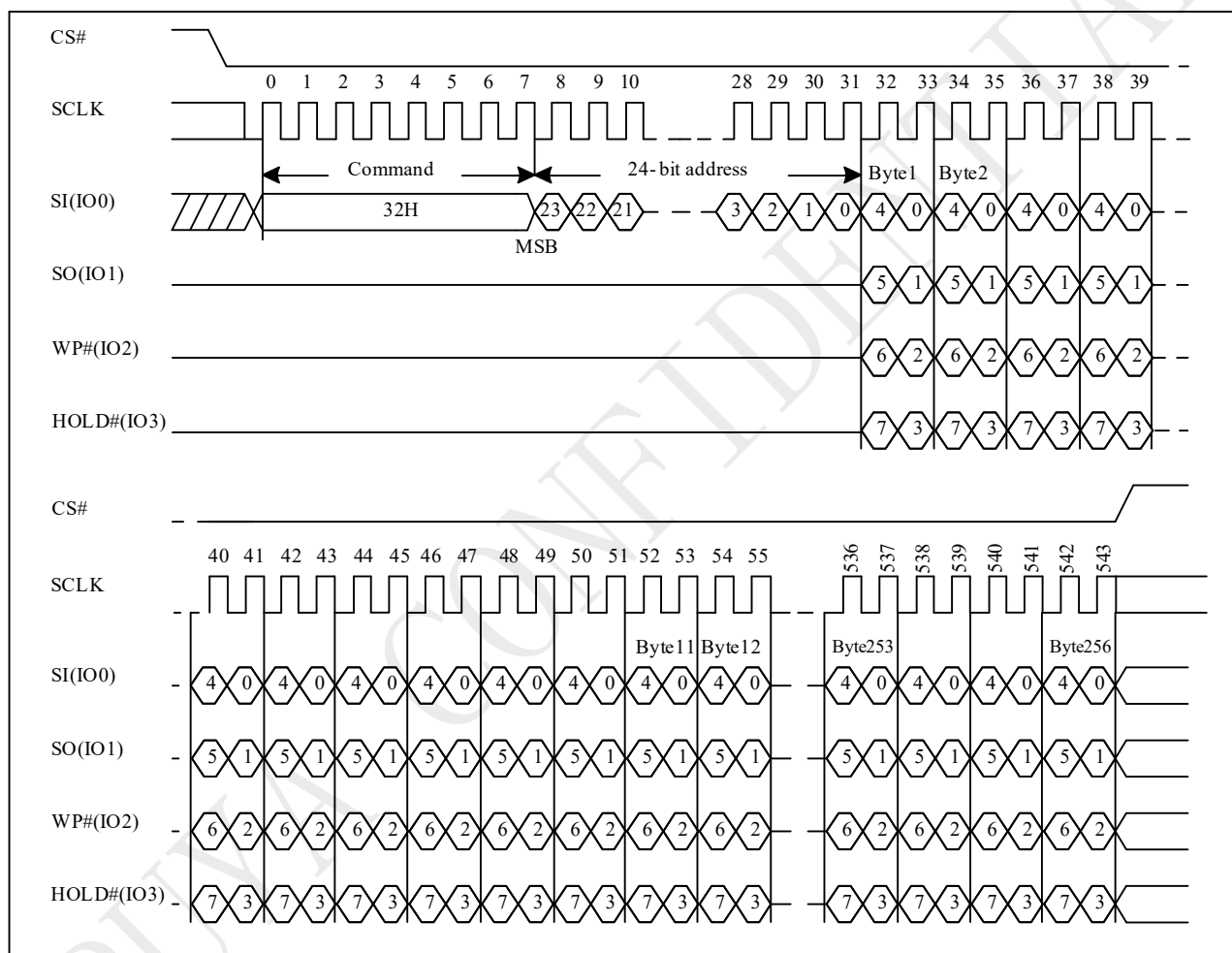
Figure 10-45 Quad Page Program (QPP) Sequence (SPI)
