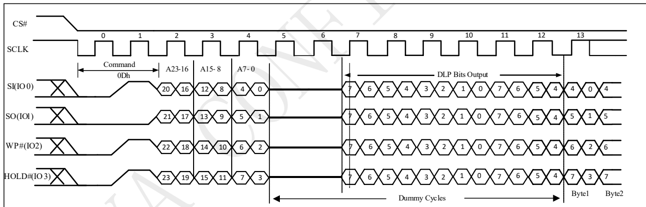
Figure 10-33h DTR 1IO Read with DLP bits output Sequence (QPI)
