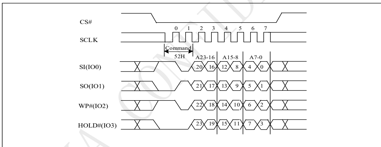
Figure 10-38a Block Erase 32K(BE32K) Sequence (QPI)
