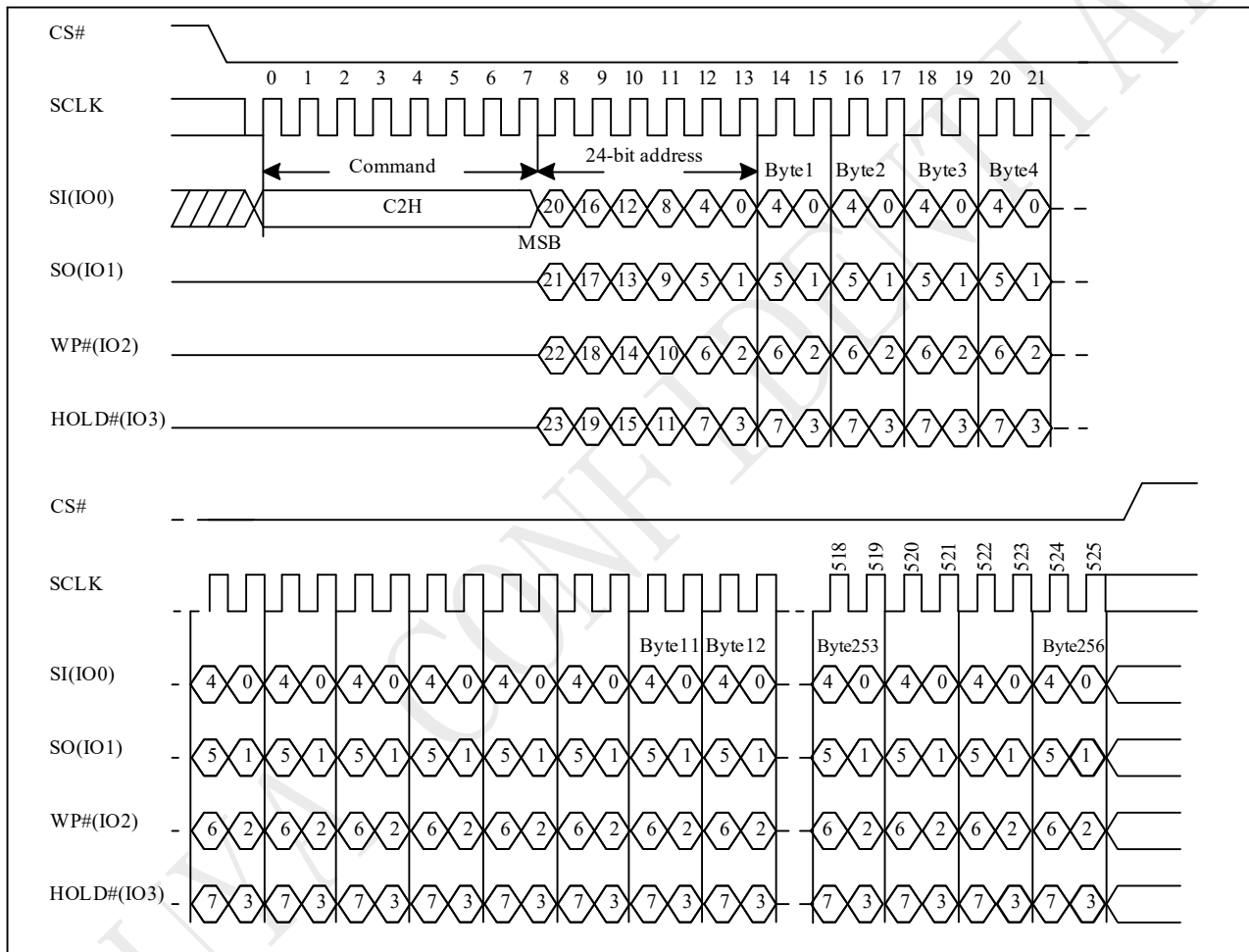
Figure 10-47 Quad Page Program (QPP) Sequence (SPI)
