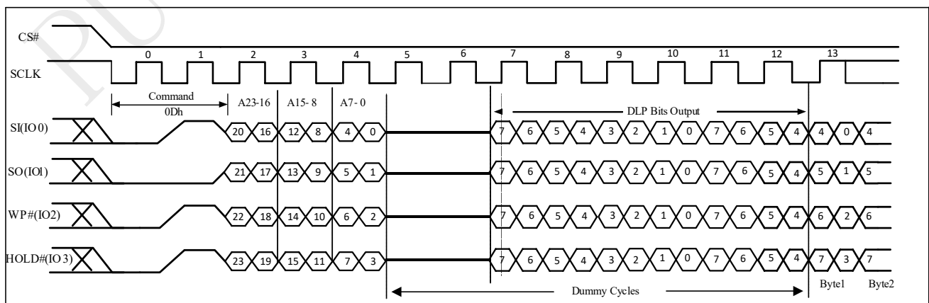
Figure 10-33k DTR 4IO Read with DLP bits output Sequence (QPI)
