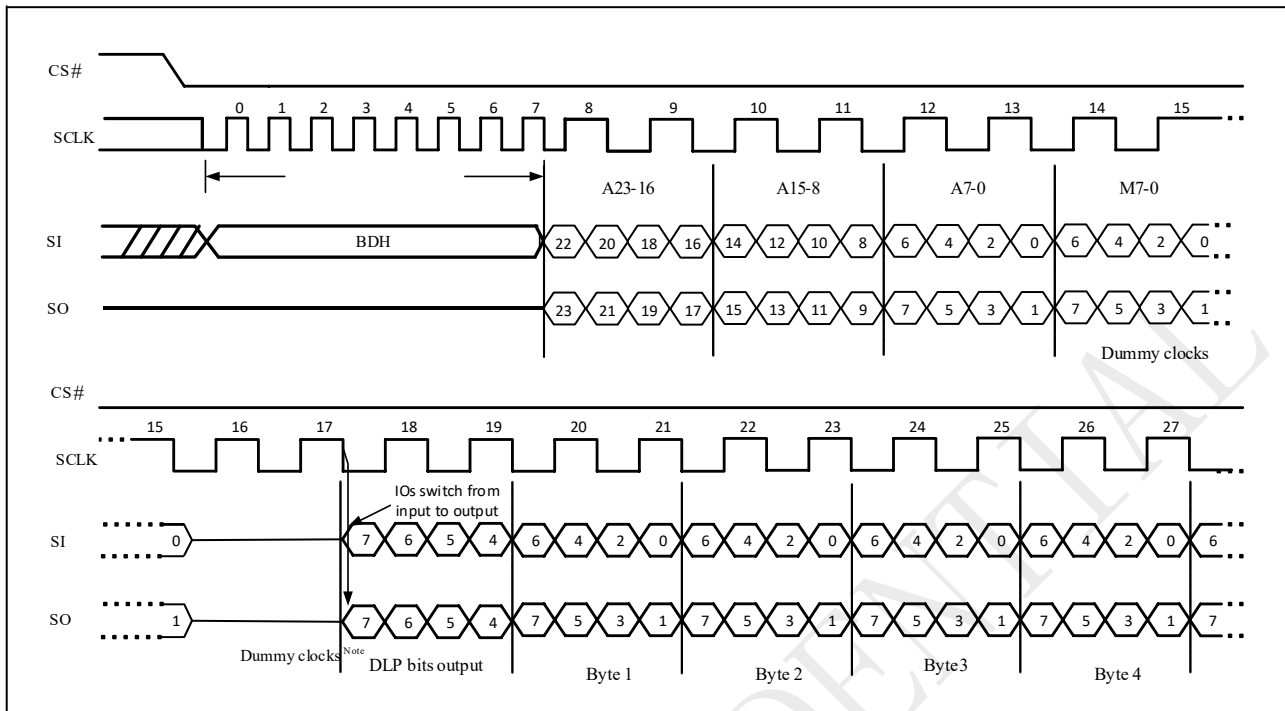
Figure 10-33i DTR 2IO Read with DLP bits output Sequence (SPI)
