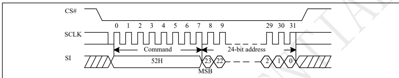
Figure 10-38 Block Erase 32K(BE32K) Sequence (SPI)
