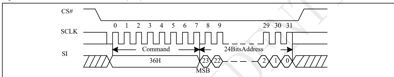
Figure 10-62 Individual Block Lock (SPI)
