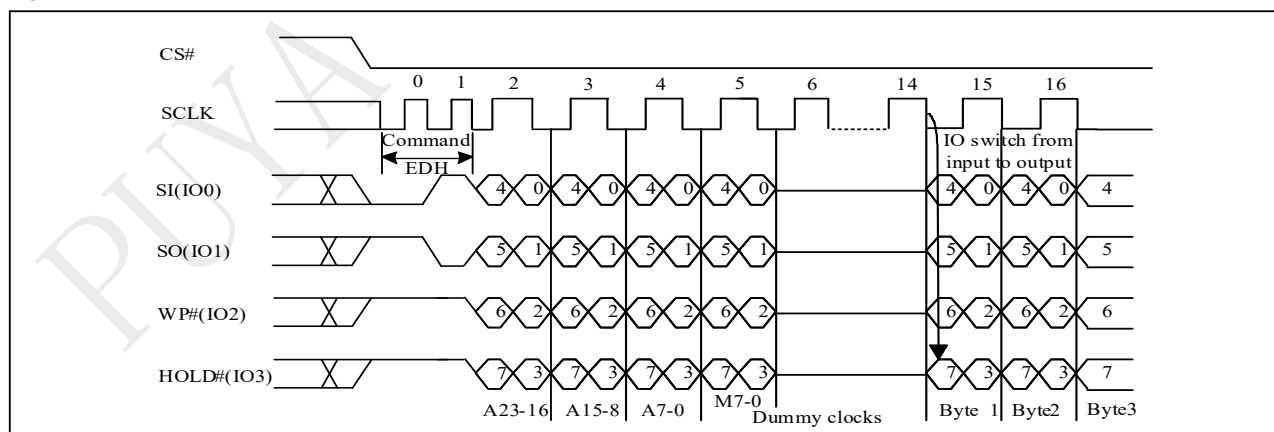
Figure 10-27b DTR 4IO Read Mode Sequence (QPI, M5-4 \neq (1,0))
