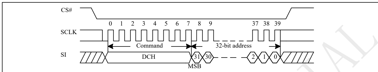
Figure 10-41 Block Erase with 4-Byte Address Sequence (SPI)
