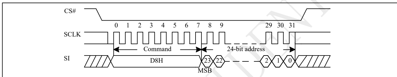
Figure 10-40 Block Erase (BE) Sequence (SPI)
